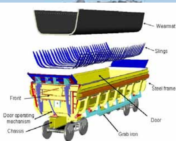
Exploded View
